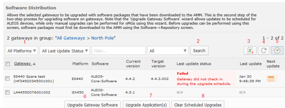
Figure 3-39: Software Distribution Screen
