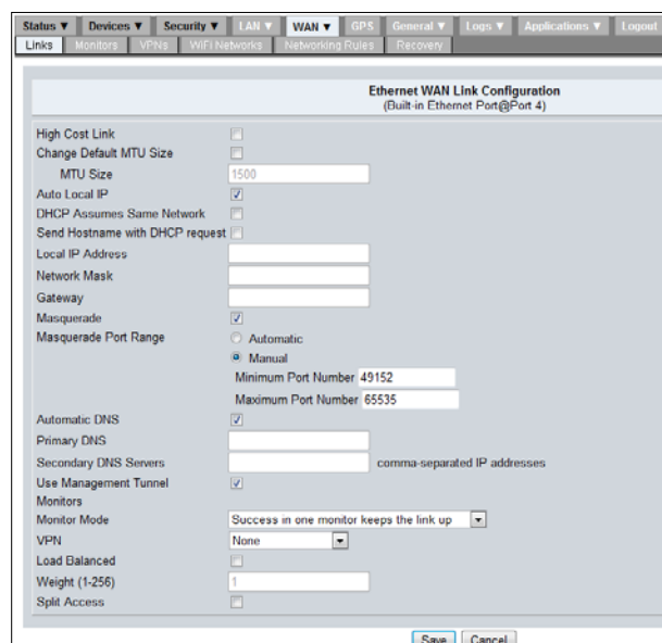
Figure 10 - Ethernet WAN Configuration Settings
