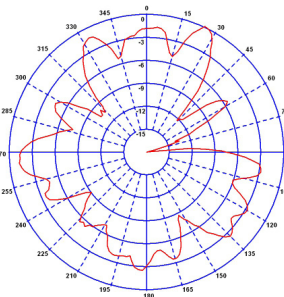
Typical H-Plane (2450MHz)
