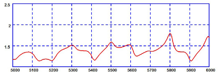
Typical VSWR WIFI elements 5GHz*
